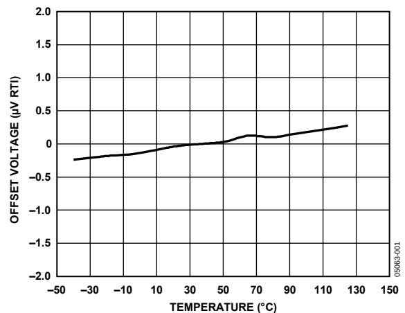
Figure 2. Relative Offset Voltage vs. Temperature
